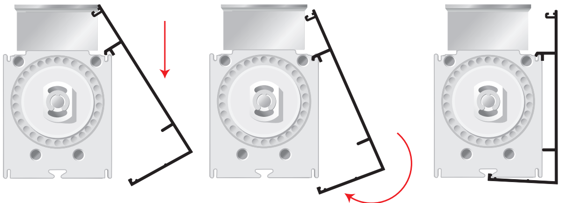
Mecho®/5 Extended Bracket
