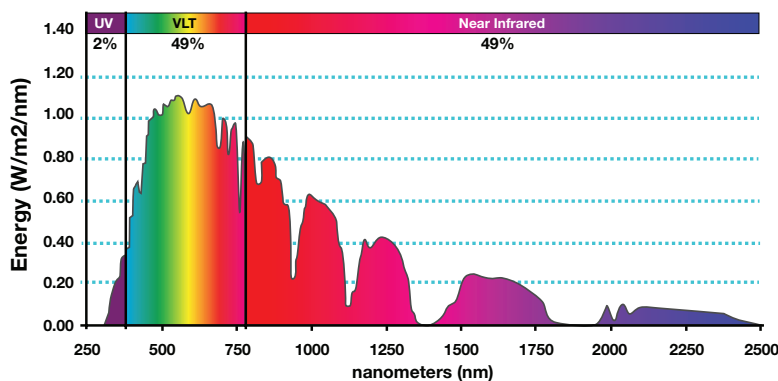
ASTM E 891 Solar Spectrum
